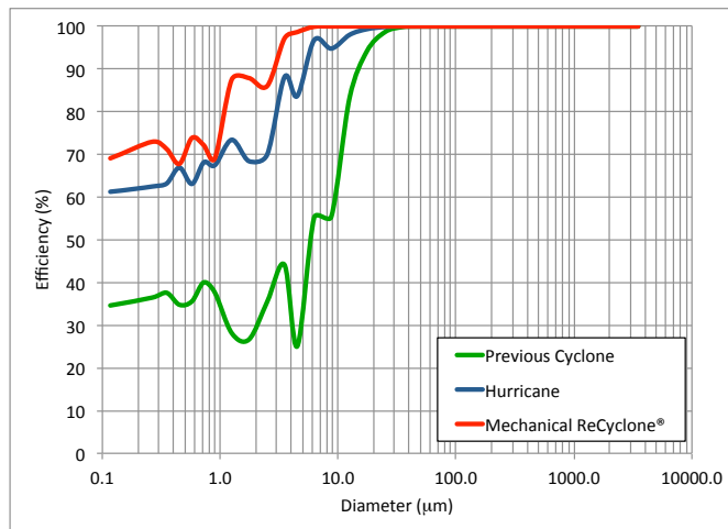
Fig. 3 – Predicted grade collection efficiency
