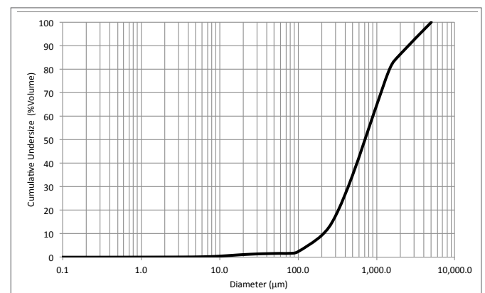
Fig. 2 – Particle Size Distribution used in simulations
