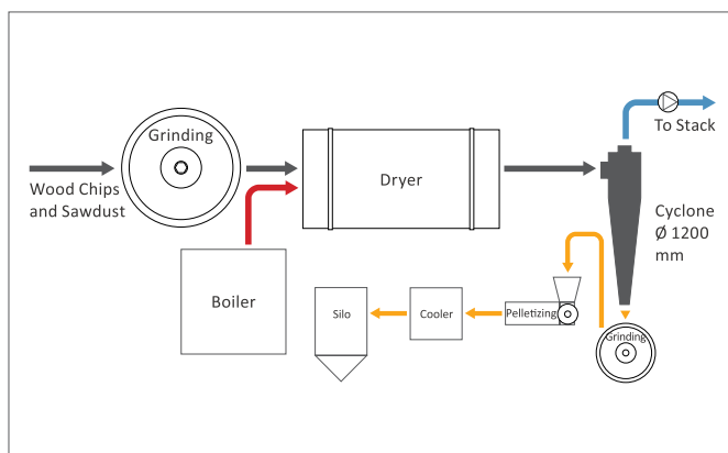
Fig. 1 – Process Scheme
